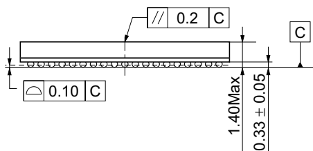
Figure D.3 Package Dimensions (BP-240A)
