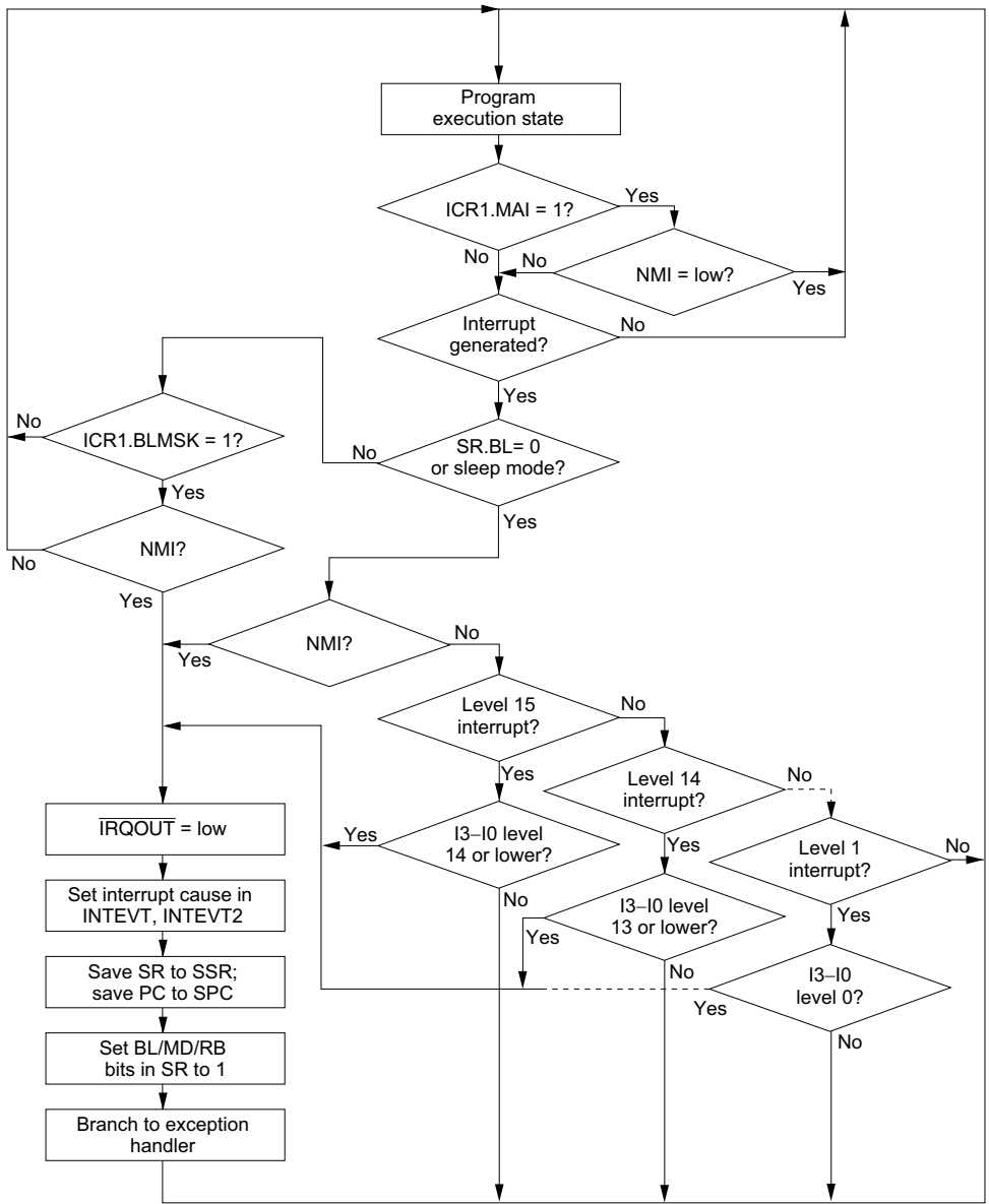
Figure 7.3 Interrupt Operation Flowchart
