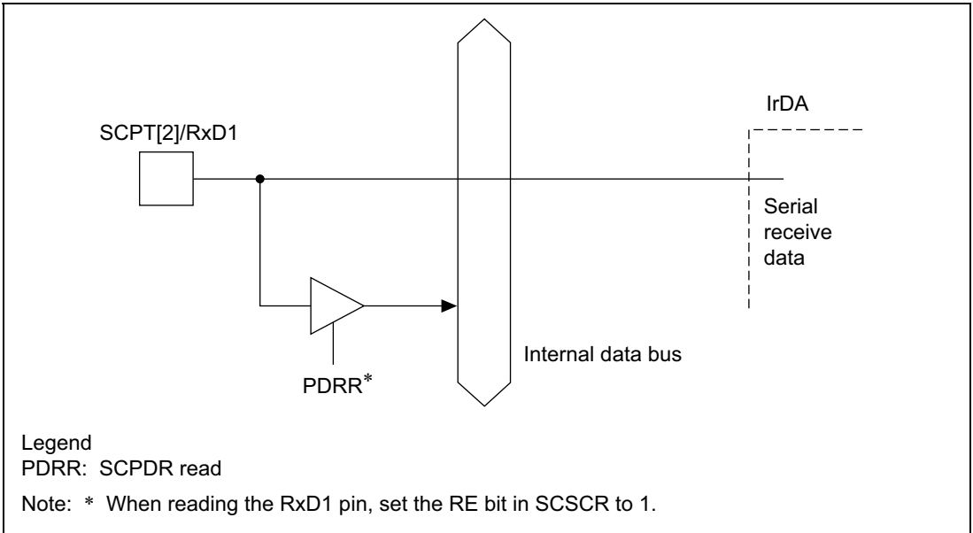
Figure 18.4 SCPT[2]/RxD1 Pin
