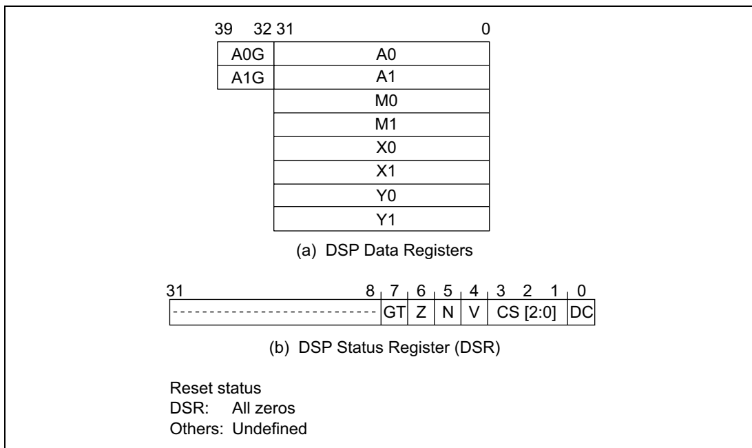
Figure 2.7 DSP Registers
