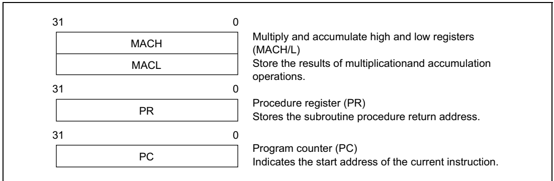
Figure 2.6 System Registers
