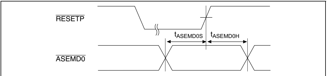
Figure 24.58 \overline{ASEMD0} Input Timing
