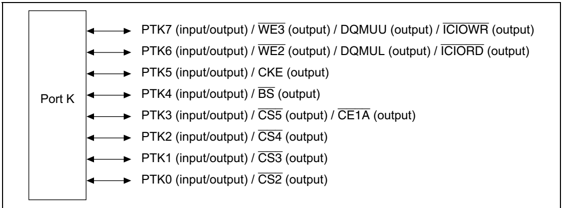
Figure 20.10 Port K
