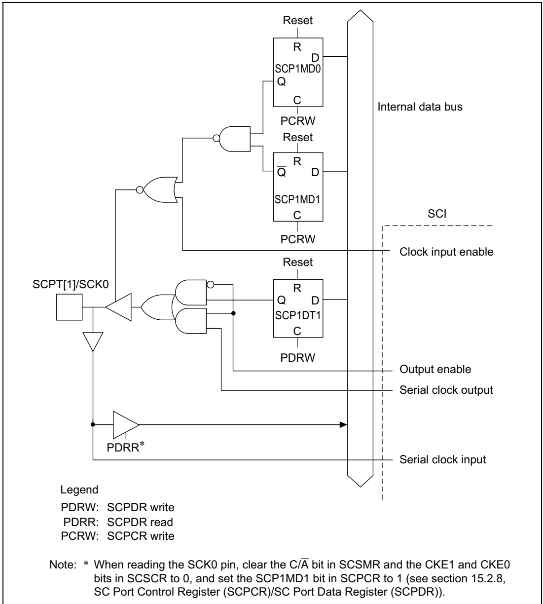
Figure 15.2 SCPT[1]/SCK0 Pin
