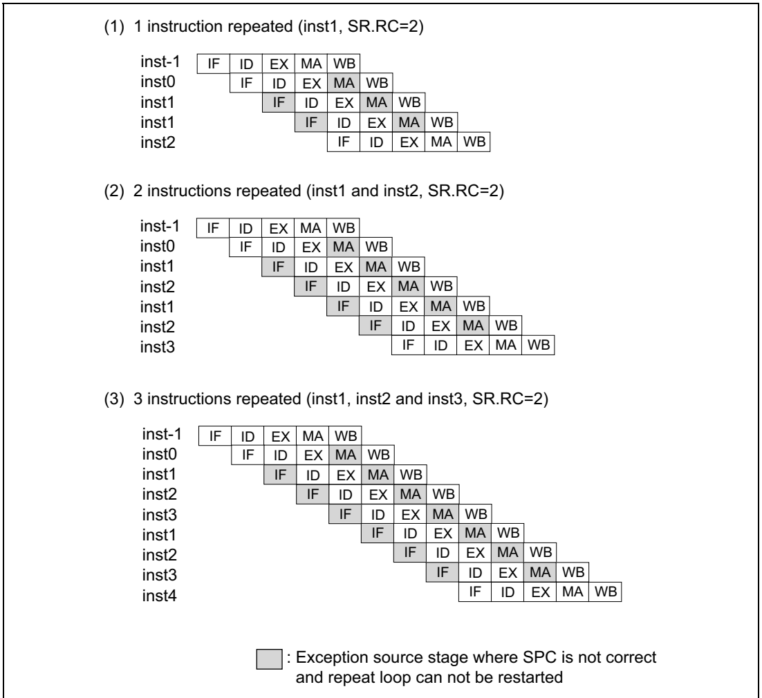
Figure 3.14 MMU Exception in Repeat Loop
