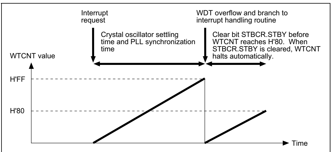
Figure 9.1 Canceling Standby Mode with STBCR.STBY
