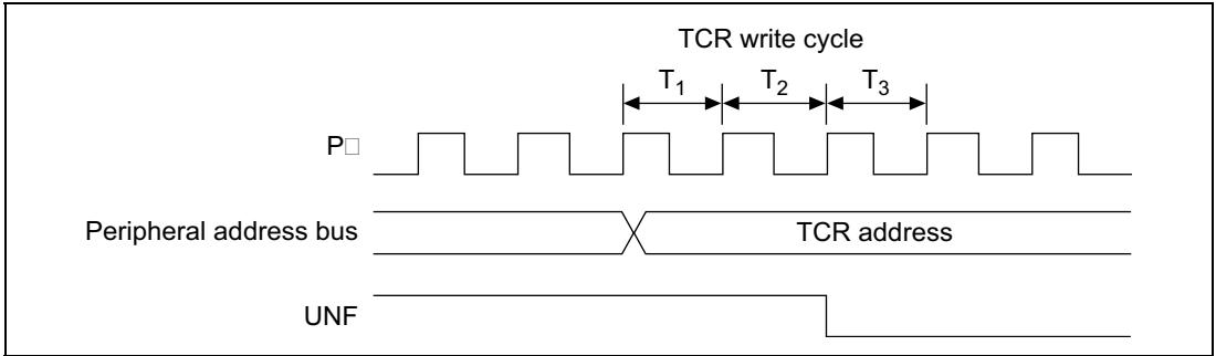
Figure 13.9 Status Flag Clearing Timing
