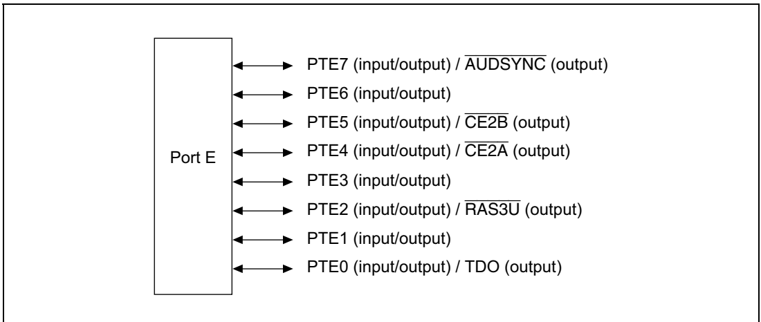
Figure 20.5 Port E
