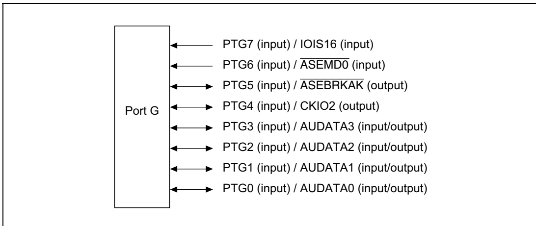
Figure 20.7 Port G
